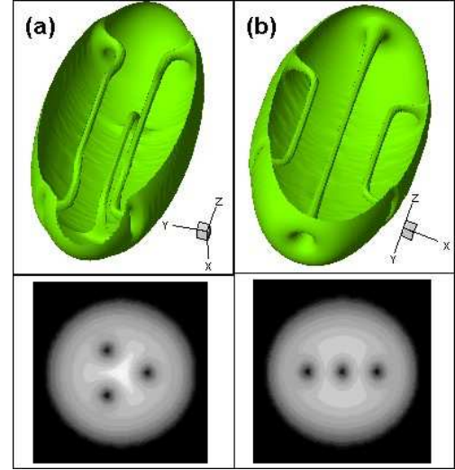
FIG. 10: Three-vortex configuration obtained for the same \Omega/\omega_x = 0.72 , from different initial conditions: 3 identical U vortices at 120^\circ (a) and 3 straight vortices in a row on the x -axis (b). Lower pictures show iso-contours of |u| in the central z = 0 cut plane.
